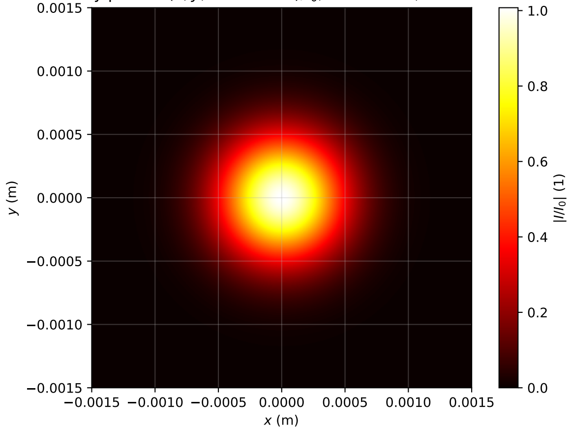
Intensity profile I(x, y, z = 0.239m)/I_0 , Pin=0.4Pcr, artificial time
